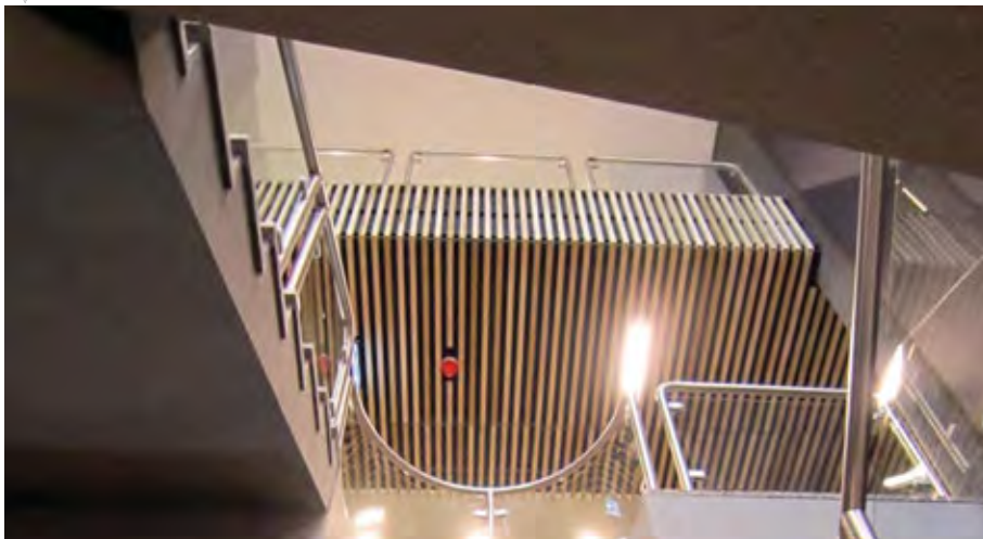
Type: 35x35 mm / 40 mm space, Yellow Poplar, clear varnish.
